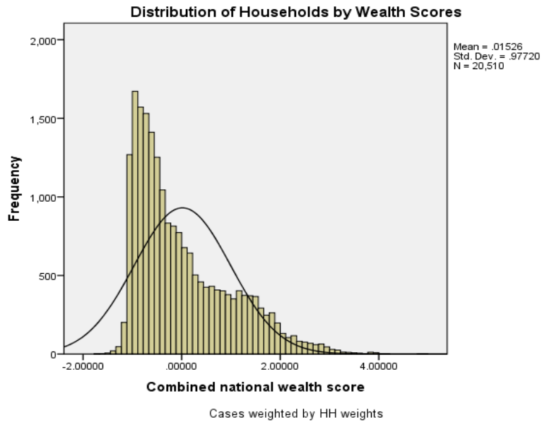
Histogram
